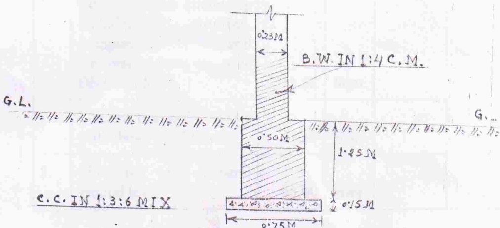
FOUNDATION-DETAIL.
